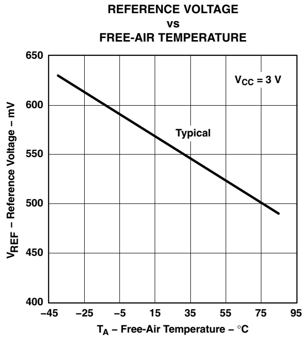
Figure 17. V_{(\text{RefVT})} vs Temperature
