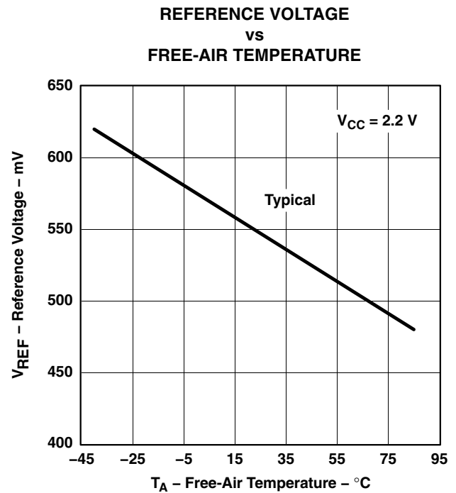
Figure 18. V_{(\text{RefVT})} vs Temperature
