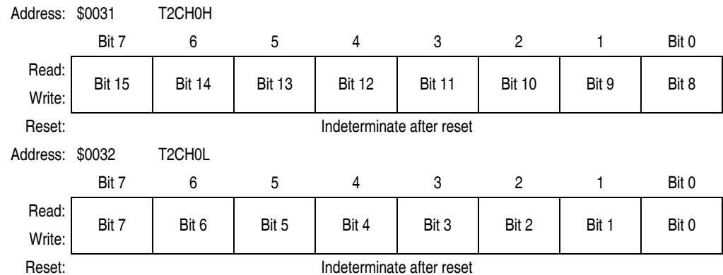
Figure 18-10. TIM2 Channel Registers (T2CH0H/L:T2CH5H/L) (Sheet 1 of 3)
