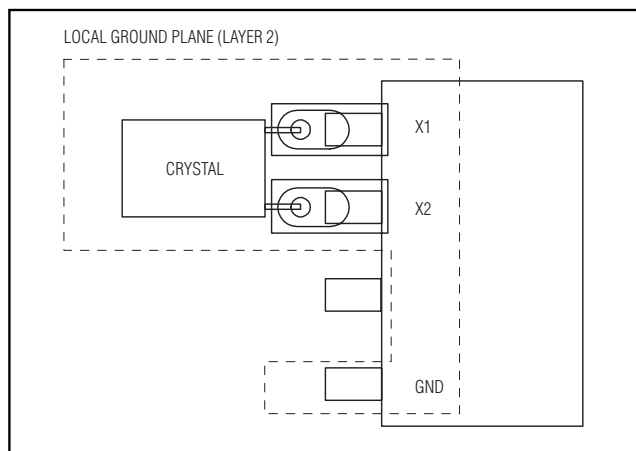
Figure 4. Layout Example
