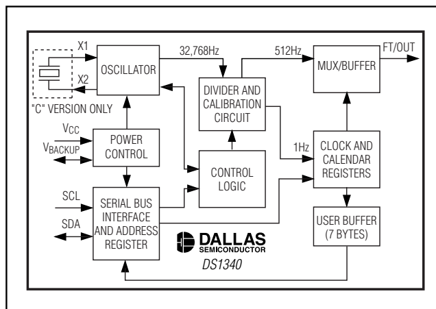
Figure 5. Functional Diagram
