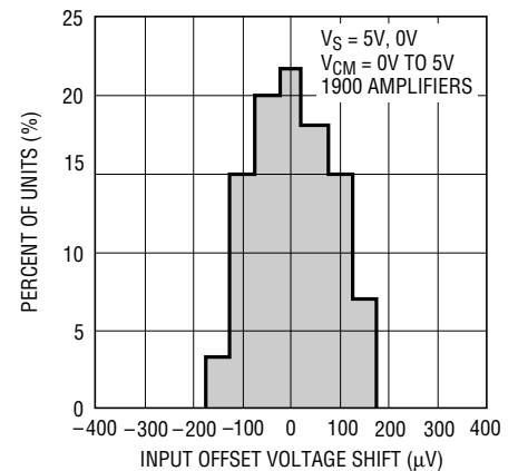
V_{OS} Shift, V_{CM} = 0\text{V} to 5\text{V}
