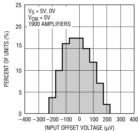
V_{OS} Distribution, V_{CM} = 5\text{V}
