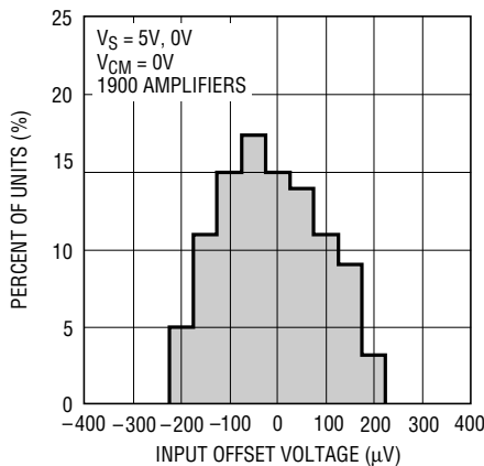
V_{OS} Distribution, V_{CM} = 0\text{V}
