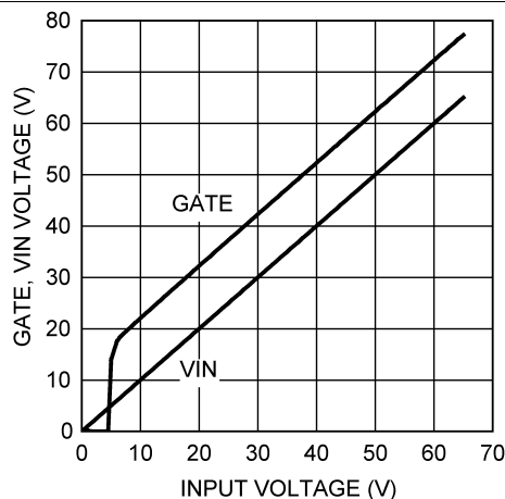
Figure 2. V_{GATE} , VIN Voltage vs Input Voltage
