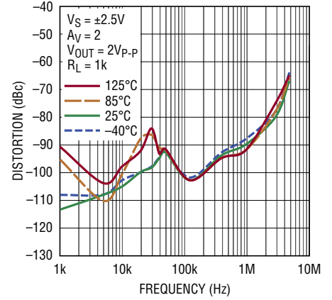
Harmonic Distortion (HD2) vs Frequency
