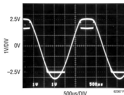
Figure 2. V_S = \pm 2.5V , A_V = 1 with Large Overdrive
