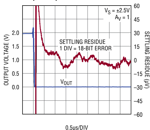
18-Bit Settling Time to 2Vp-p Output Step
