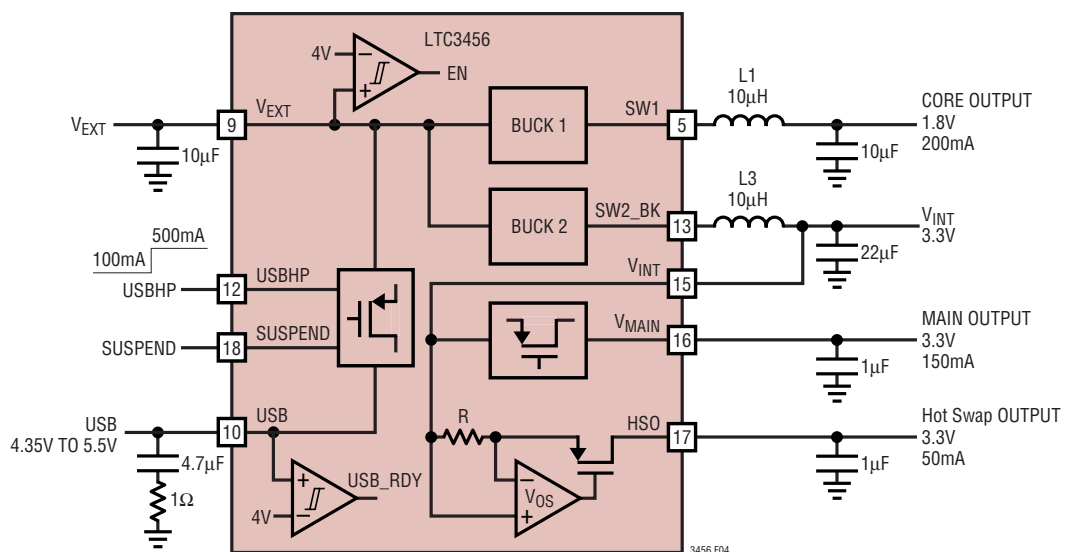
Figure 4. USB-Powered LTC3456
