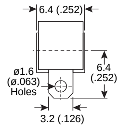
Solder Terminal
