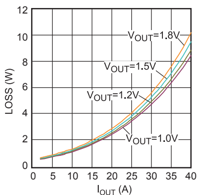
Device Loss vs. Output Current
