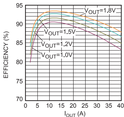
Device Efficiency vs. Output Current
