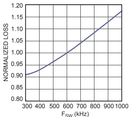
Normalized Power Loss vs. Switching Frequency
