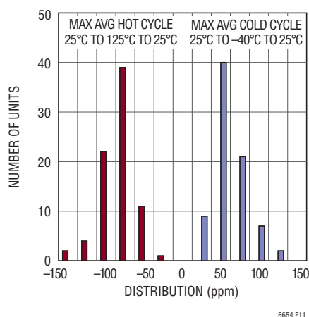
Figure 11a. LT6654 S6 Thermal Hysteresis -40^{\circ}\text{C} to 125^{\circ}\text{C}
