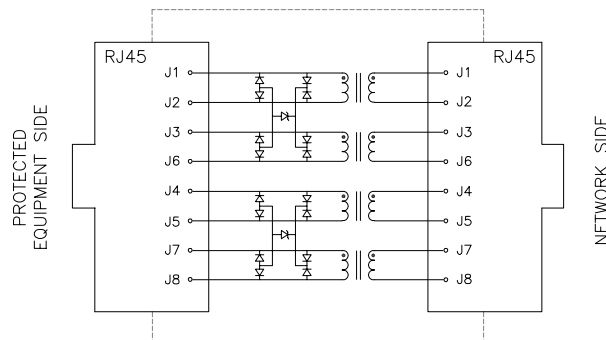
Circuit B
