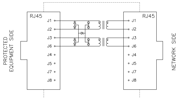
Circuit A
