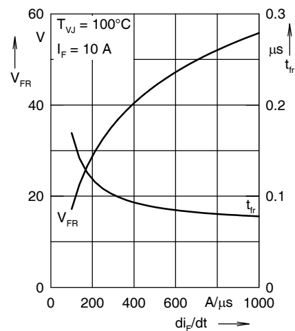
Fig. 23. Peak forward voltage V_{FR} and t_{rr}
