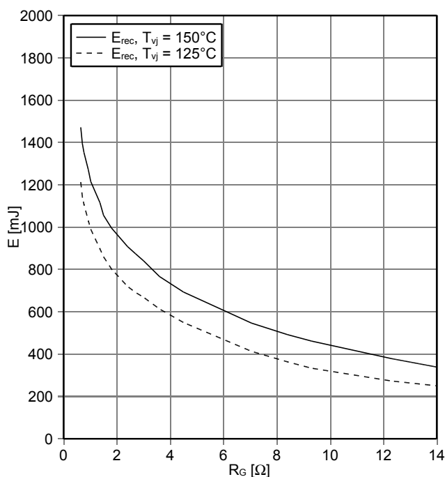
Schaltverluste Diode, Revers (typisch) switching losses Diode, Reverse (typical) E_{rec} = f(R_G) I_F = 1000 A , V_{CE} = 1800 V
