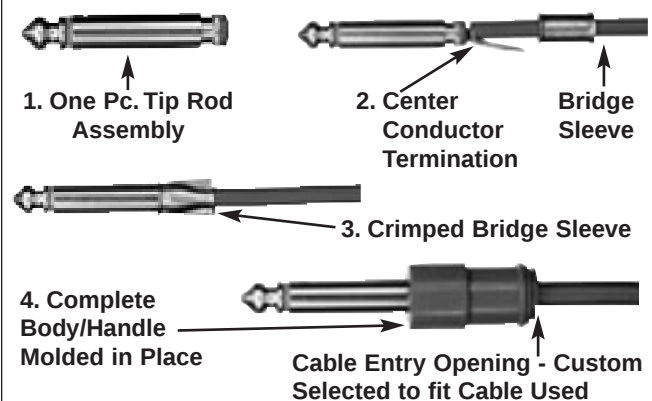
FIGURE 1: MOLDED CABLE MANUFACTURING STEPS FOR 1/4" LITTEL PLUG®
