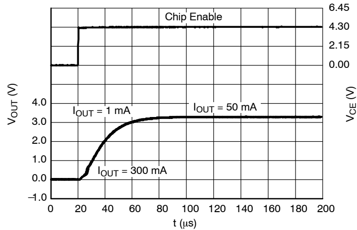
Figure 82. Start-up, 3.3 V Version, V_{IN} = 4.3\text{ V}
