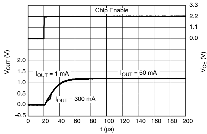
Figure 80. Start-up, 1.2 V Version, V_{IN} = 2.2\text{ V}
