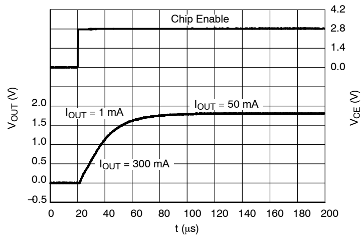
Figure 81. Start-up, 1.8 V Version, V_{IN} = 2.8\text{ V}
