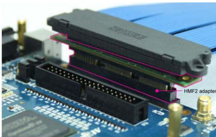
DE2-115 linking with DE2-115
