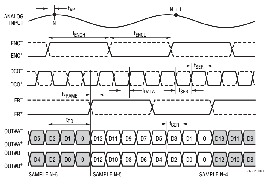
2-Lane Output Mode, 16-Bit Serialization*
