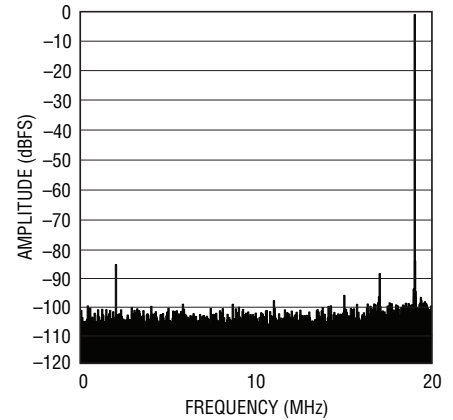
LTC2171-14: 8k Point FFT, f_{IN} = 139\text{MHz} , -1\text{dBFS} , 40\text{Mpsps}
