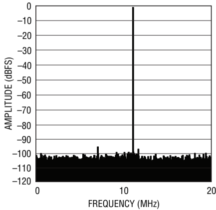
LTC2171-14: 8k Point FFT, f_{IN} = 29\text{MHz} , -1\text{dBFS} , 40\text{Mpsps}
