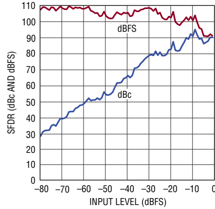
LTC2172-14: SFDR vs Input Level, f_{IN} = 70\text{MHz} , 2V Range, 65Msps
