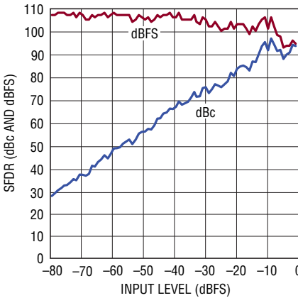
LTC2170-14: SFDR vs Input Level, f_{IN} = 70\text{MHz} , 2V Range, 25Msps
