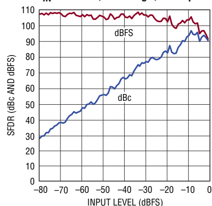
LTC2171-14: SFDR vs Input Level, f_{IN} = 70\text{MHz} , 2\text{V} Range, 40\text{Mpsps}
