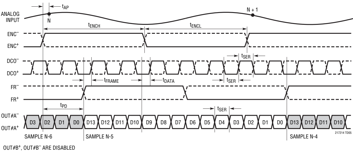
1-Lane Output Mode, 14-Bit Serialization
