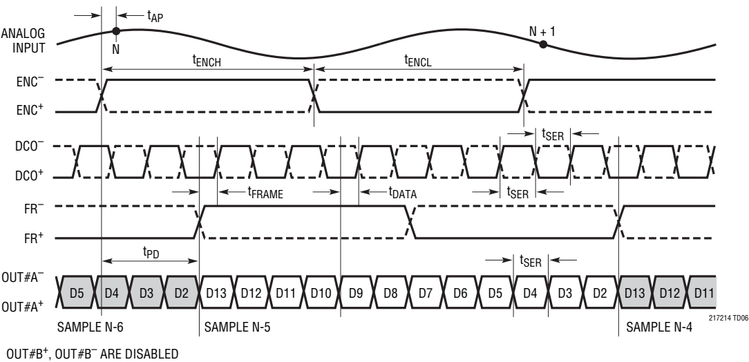
1-Lane Output Mode, 12-Bit Serialization
