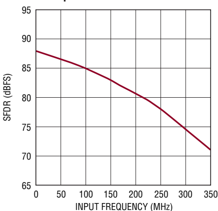
LTC2171-14: SFDR vs Input Frequency, -1\text{dBFS} , 2\text{V} Range, 40\text{Mpsps}
