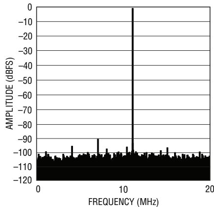
LTC2171-14: 8k Point FFT, f_{IN} = 69\text{MHz} , -1\text{dBFS} , 40\text{Mpsps}
