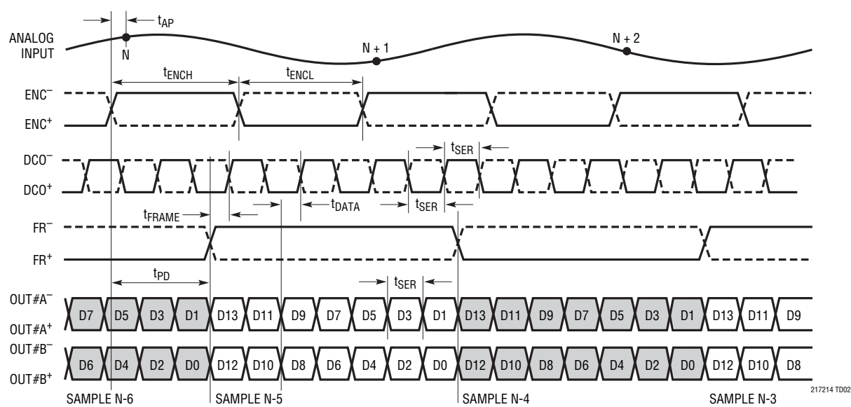
2-Lane Output Mode, 14-Bit Serialization
