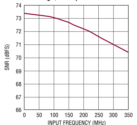
LTC2171-14: SNR vs Input Frequency, -1\text{dBFS} , 2\text{V} Range, 40\text{Mpsps}
