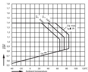
Relay operation voltage vs. ambient temperature
