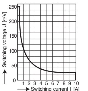
Maximum switching power curve
