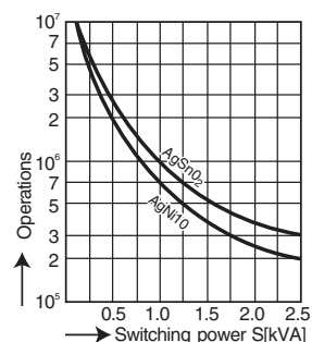
Mechanical life
