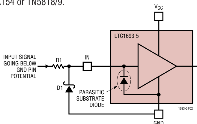
Figure 2. Input Protection Against Negative Input Signals
