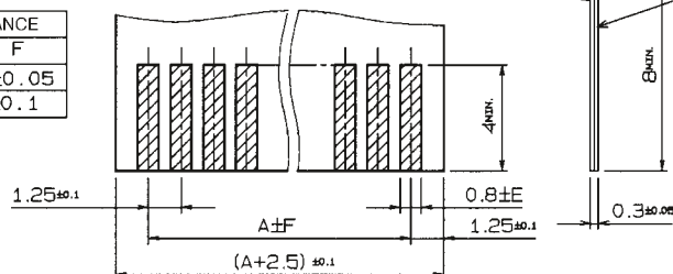
適合FPC, FFC寸法 APPLICABLE FPC/FFC
