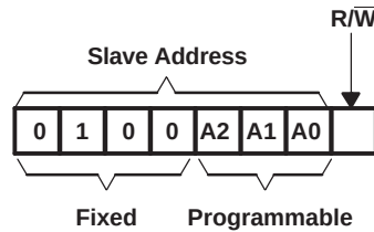
Figure 22. PCA9555 Address
