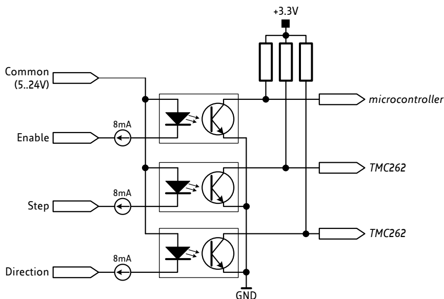
Figure 3.8 Step/Dir/Enable inputs
