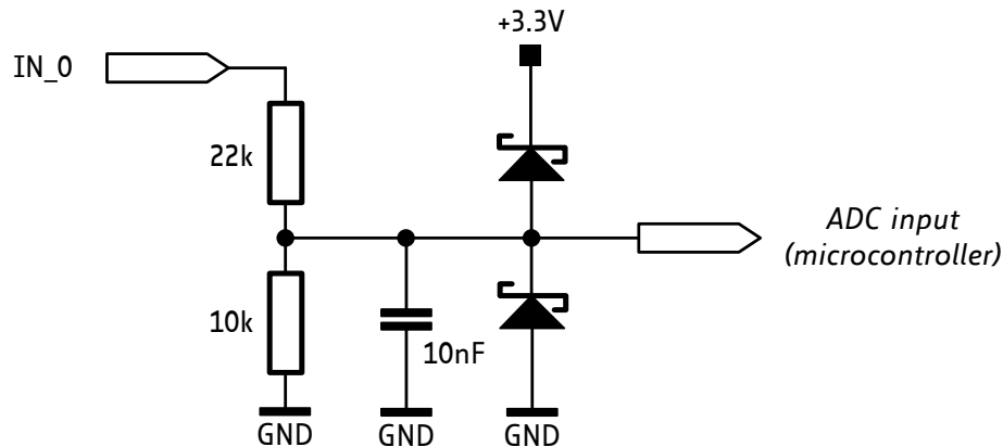
Figure 3.6 General purpose inputs (simplified input circuit)
