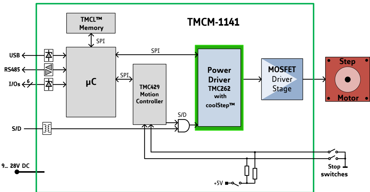
Figure 7.1 Main parts of the TMC1141
