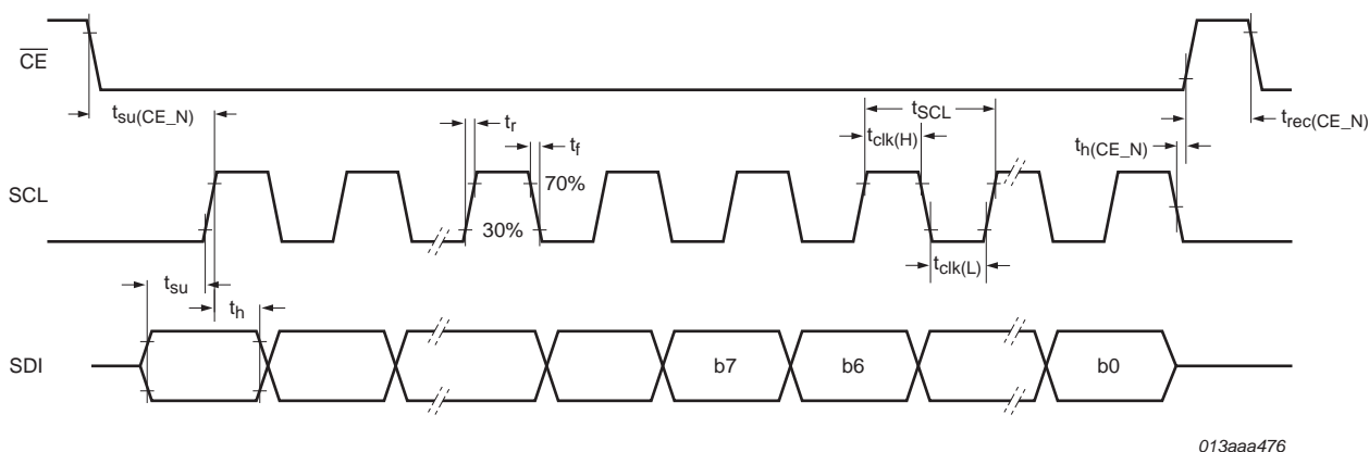
Fig 50. SPI-bus timing
