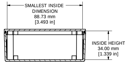
SECTION G-G
