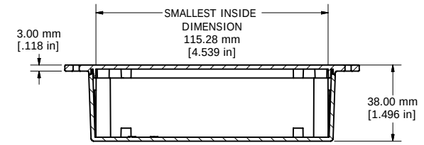
SECTION H-H
