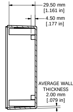
SECTION J-J
