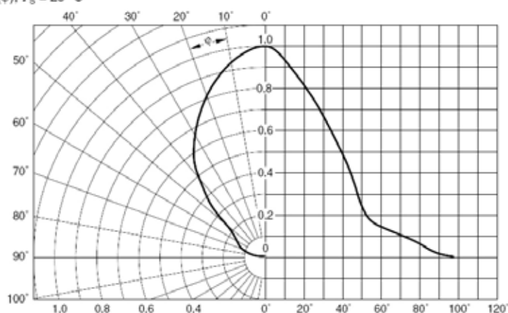
Radiation Characteristic
