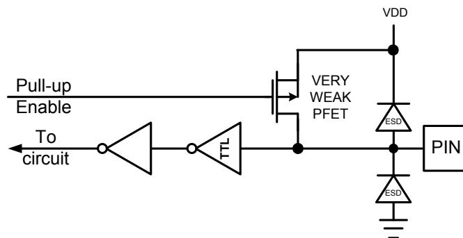
Figure 42: \overline{\text{PRES}} Input Circuit
