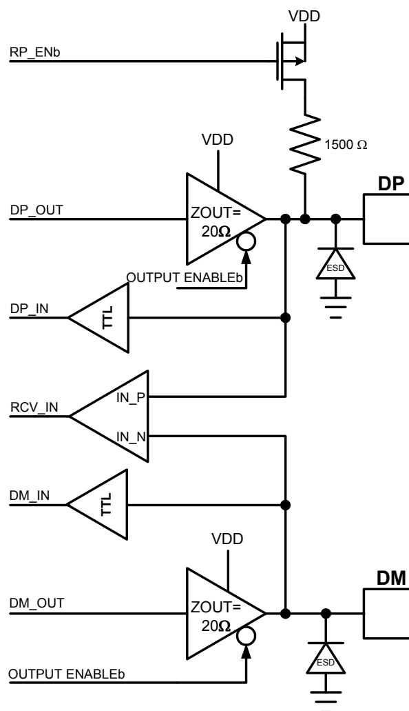
Figure 43: USB Circuit
