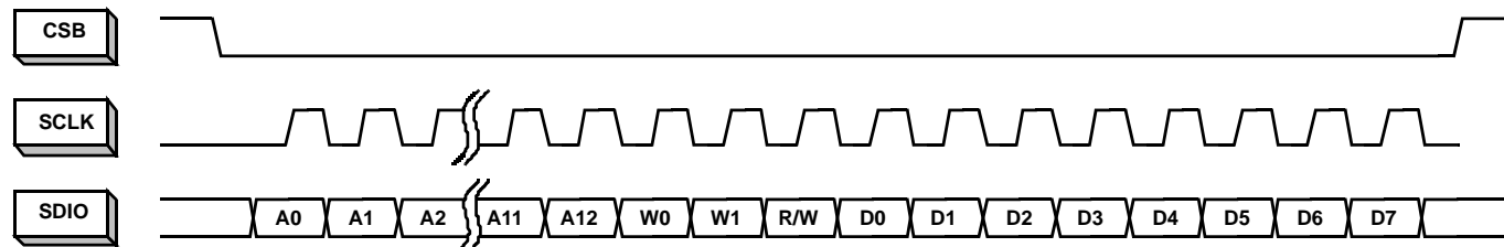
FIGURE 40. LSB-FIRST ADDRESSING
