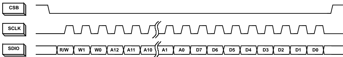
FIGURE 39. MSB-FIRST ADDRESSING
