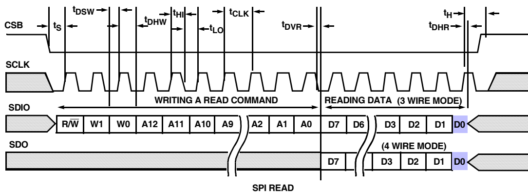
FIGURE 42. SPI READ
