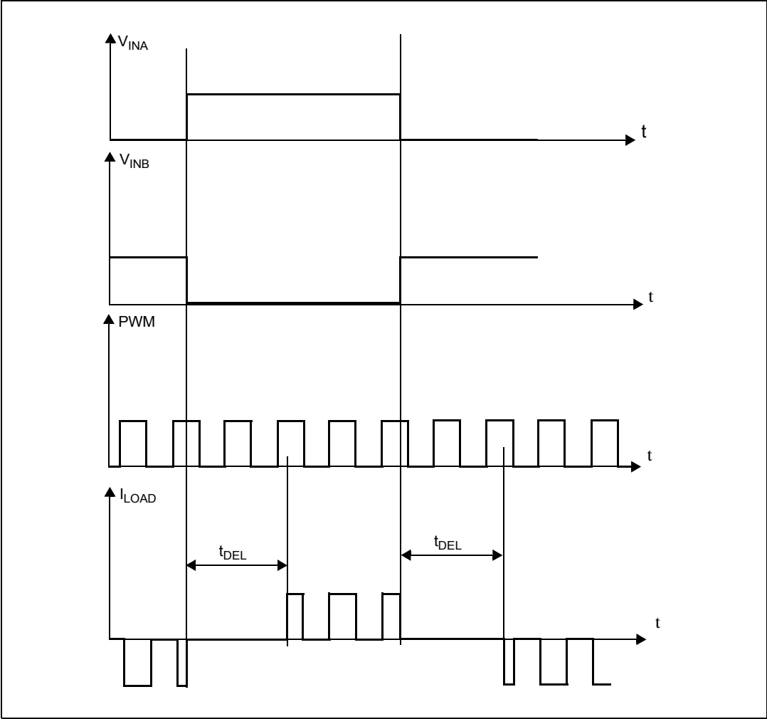
Figure 4. Definition of the delay time measurement
