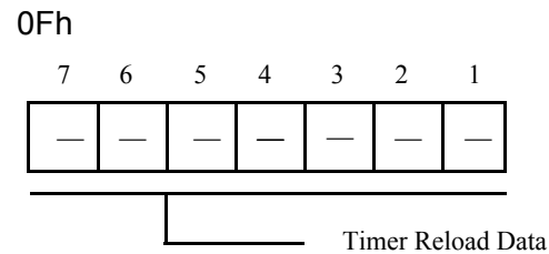
Figure 40. Timer Reload Register
