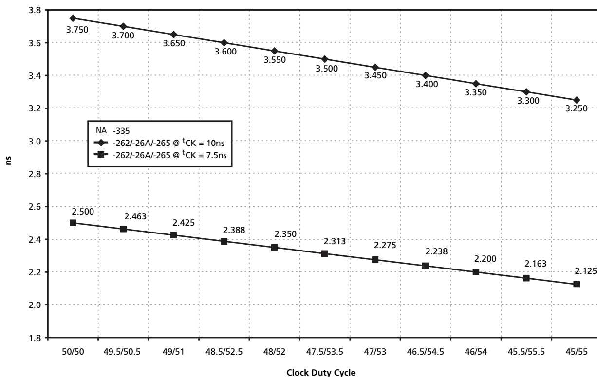
Figure 7: Derating Data Valid Window ( t_{QH} - t_{DQSQ} )
