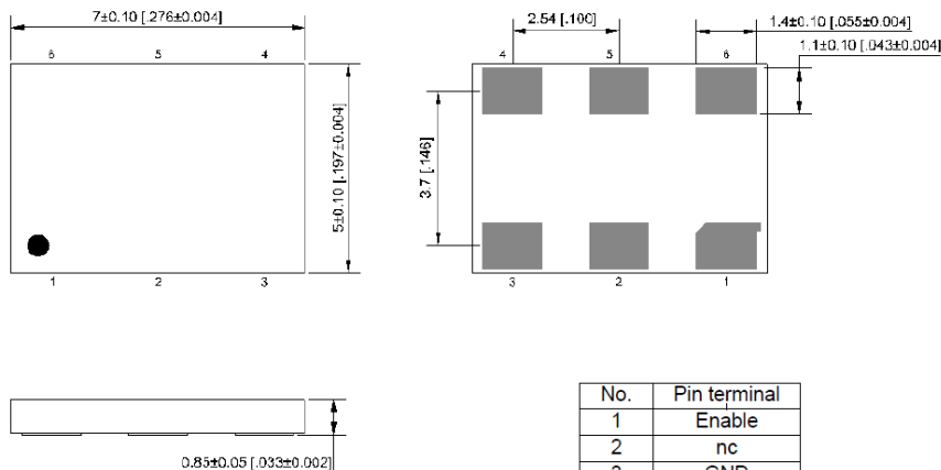
External Dimensions
