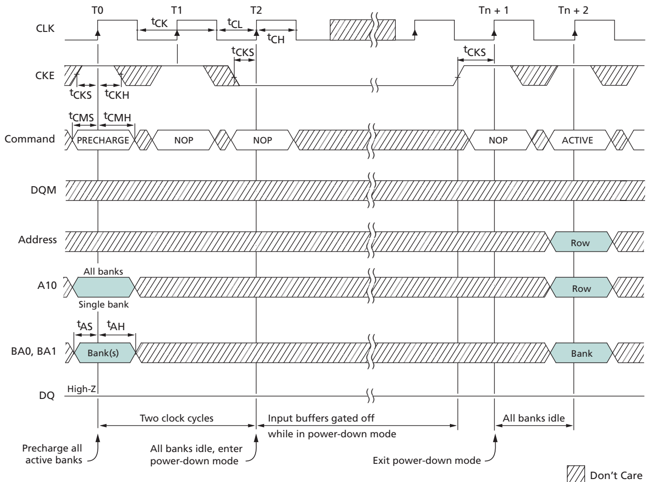
Figure 48: Power-Down Mode
