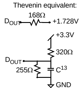
Figure B: 3.3V Output load
