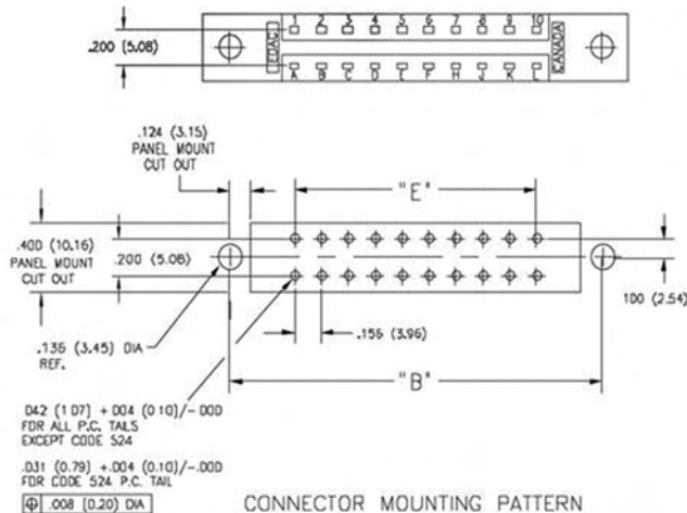
CONNECTOR MOUNTING PATTERN
