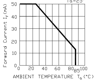
Forward Current Derating Curve T_a=25^\circ
