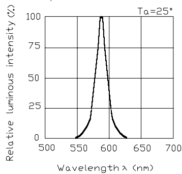
Spectrum Distribution T_a=25^\circ
