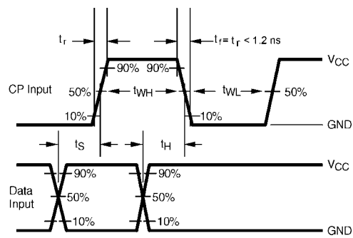
FIGURE 5. AC Waveforms
