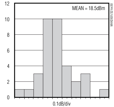
PA OUTPUT POWER HISTOGRAM FOR 1.1V POWER DETECTOR OUTPUT
