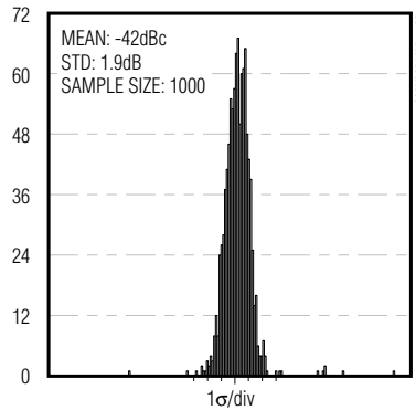
HISTOGRAM: Tx SIDEBAND SUPPRESSION
