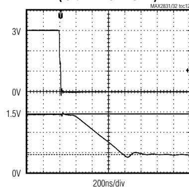
Rx RSSI STEP RESPONSE (-32dB LNA GAIN STEP)
