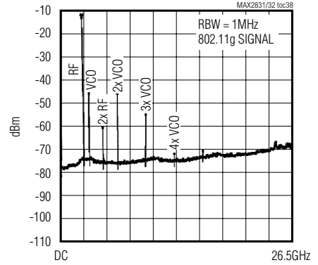
Tx OUTPUT SPURS (MAX2832 ONLY)
