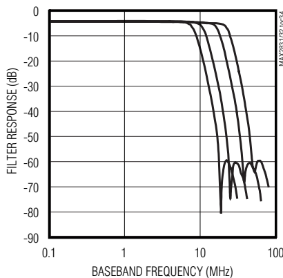
Tx BASEBAND FREQUENCY RESPONSE
