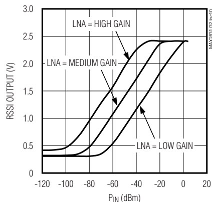
Rx RSSI OUTPUT vs. INPUT POWER
