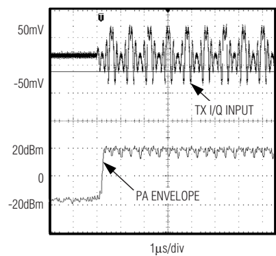
PA OUTPUT ENVELOPE RESPONSE
