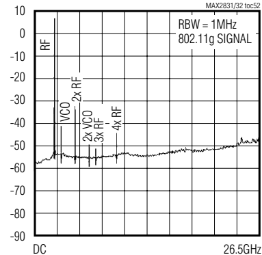
Tx OUTPUT SPURS
