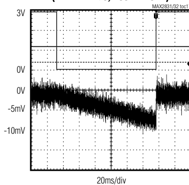
I/Q OUTPUT DC ERROR DROOP ( RxHP = 1 \rightarrow 0 ; 100Hz MODE)
