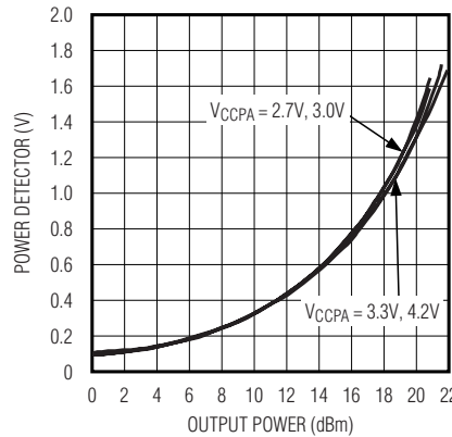
POWER DETECTOR OVER SUPPLY VOLTAGE
