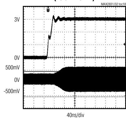
Rx BB VGA SETTLING RESPONSE (+8 GAIN STEP)
