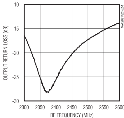
PA OUTPUT RETURN LOSS vs. RF FREQUENCY
