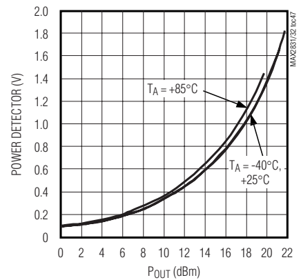
POWER DETECTOR OVER TEMPERATURE
