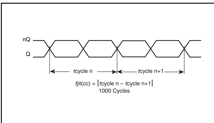
Cycle-to-Cycle Jitter
