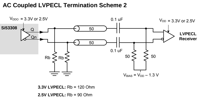
Figure 7. LVPECL Output Termination
