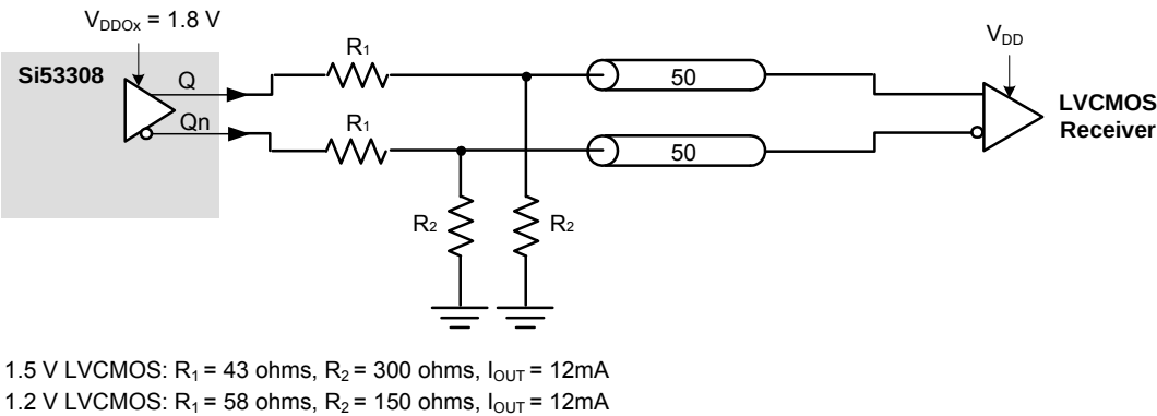
Figure 10. 1.5 V and 1.2 V LVC MOS Low-Voltage Output Termination
