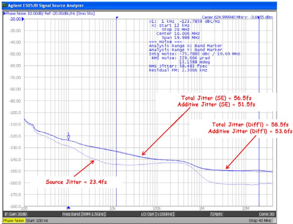
Figure 14. Differential Total Jitter (625 MHz)
