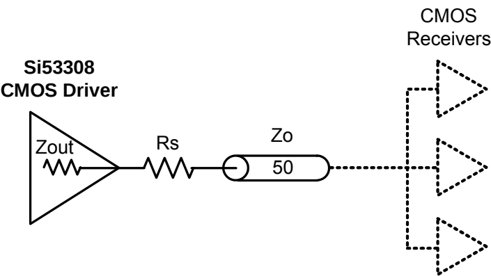
Figure 9. LVC MOS Output Termination
