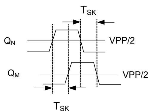
Output-Output Skew
