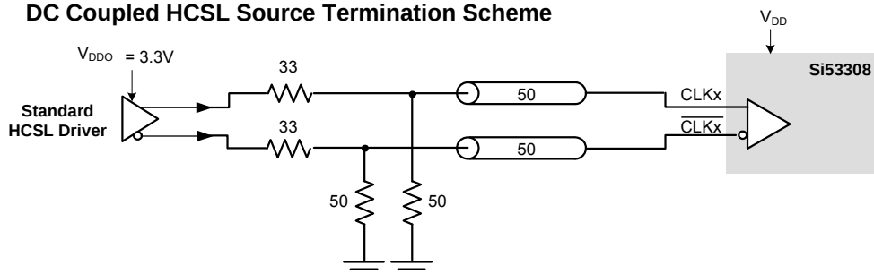
Figure 5. Differential DC-Coupled Input Terminations
