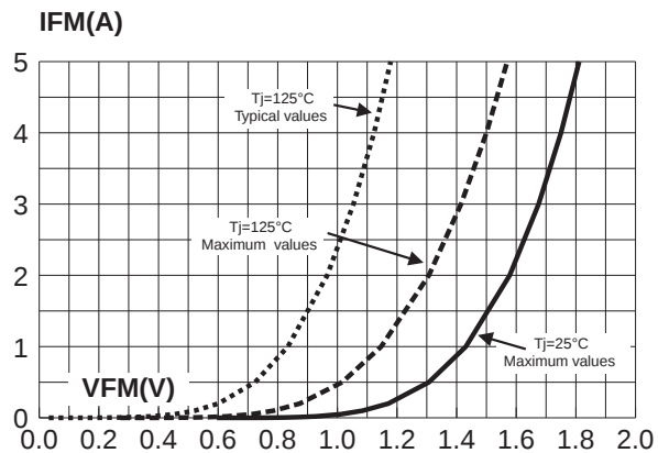
Fig. 4-1: Forward voltage drop versus forward current (low level).
