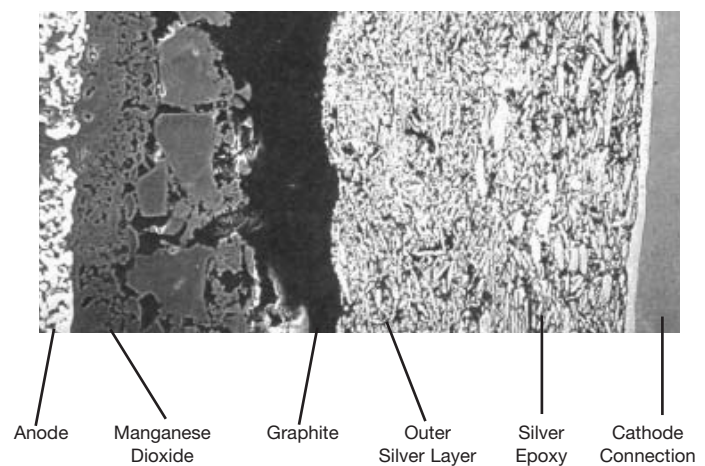
Figure 5. Cathode Termination
