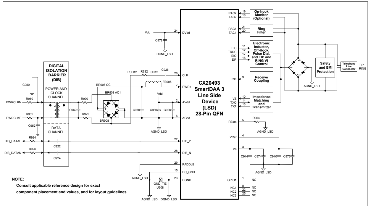
Figure 3-3. CX20493 LSD 28-Pin QFN Hardware Interface Signals
