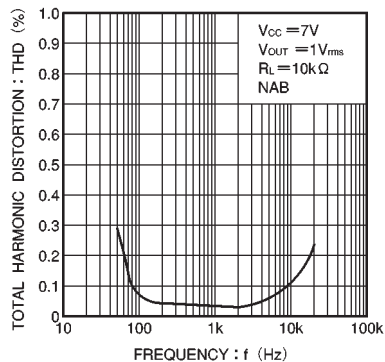
Fig. 12 Total harmonic distortion vs. frequency
