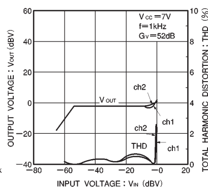
Fig. 17 ALC characteristics
