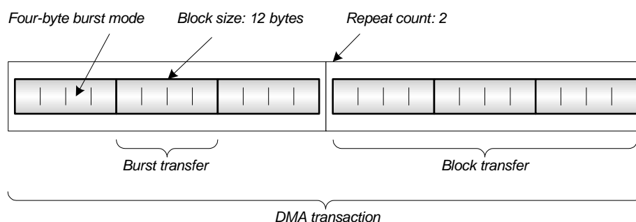
Figure 5-1. DMA transaction.
