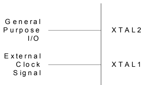
Figure 7-3. External Clock Drive Configuration
