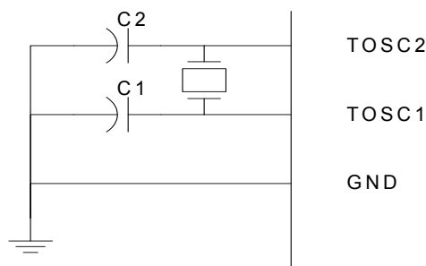
Figure 7-4. 32.768 kHz crystal oscillator connection
