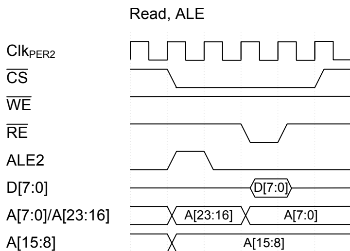
Figure 33-14. Read, ALE
