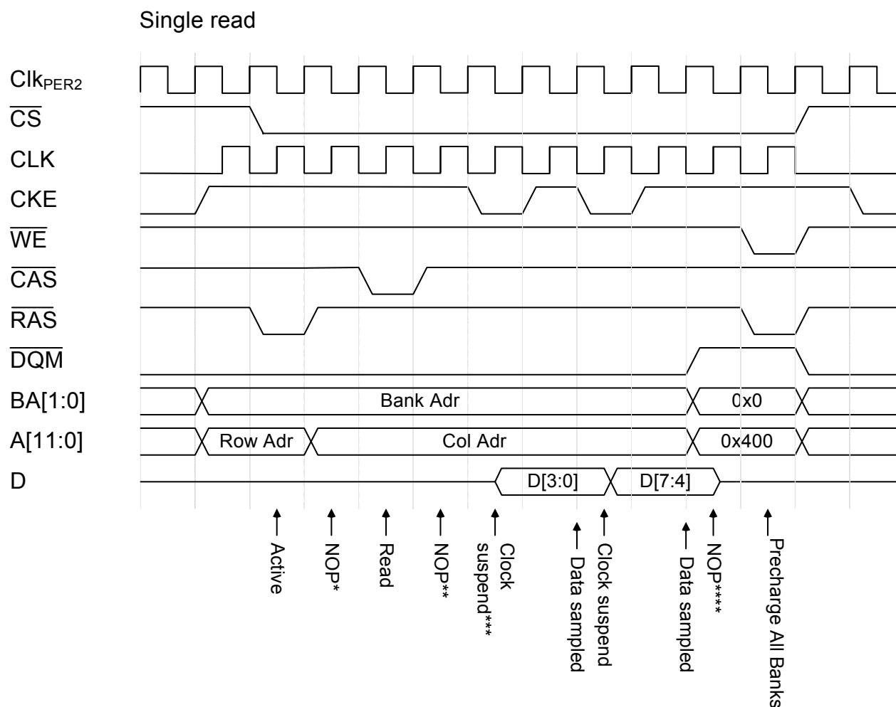
Figure 33-48. Single read
