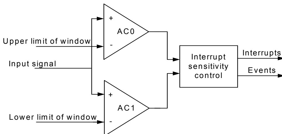
Figure 27-2. Analog Comparator Window Mode
