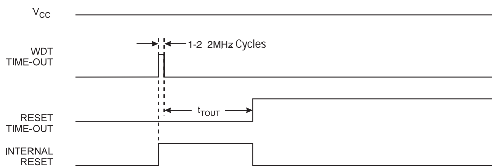
Figure 9-6. Watchdog reset.
