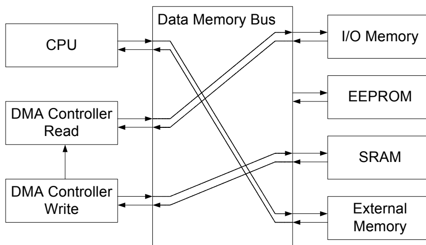
Figure 4-3. Bus Access
