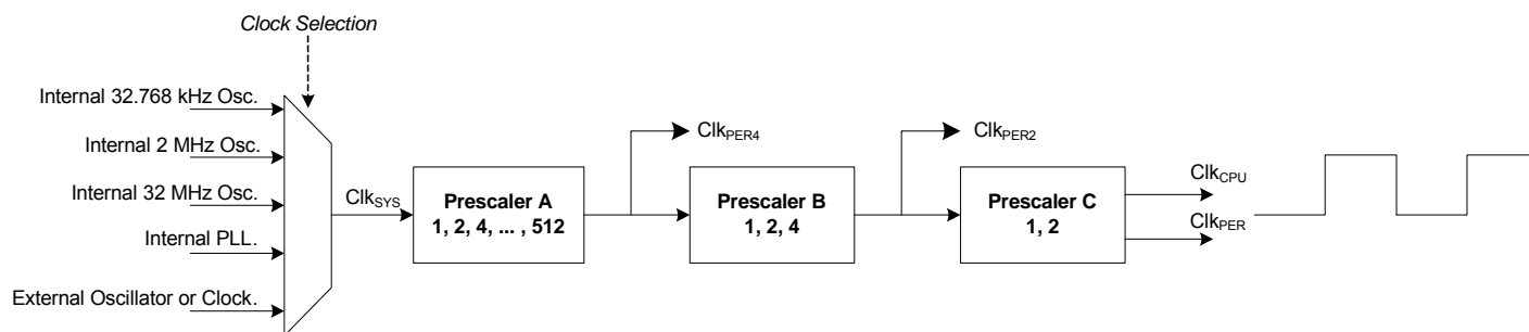
Figure 7-5. System Clock Selection and Prescalers
