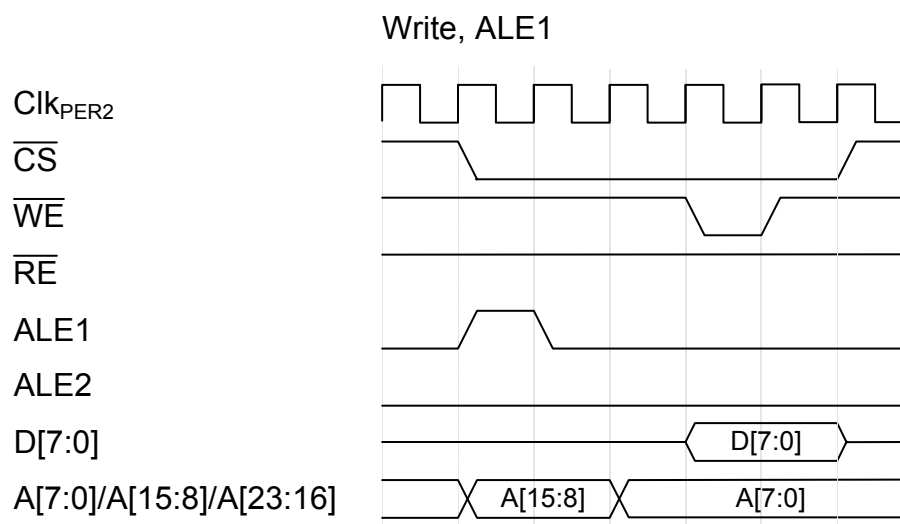
Figure 33-6. Write, ALE1
