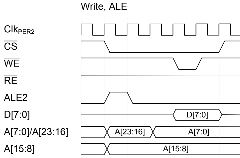
Figure 33-12. Write, ALE
