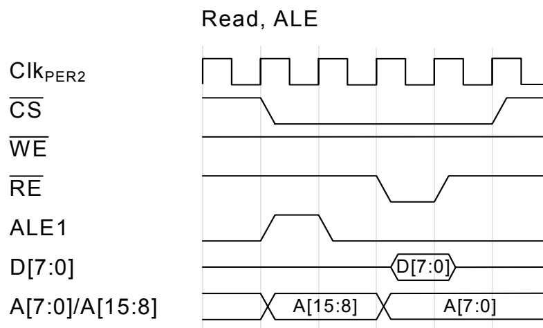
Figure 33-4. Read, ALE
