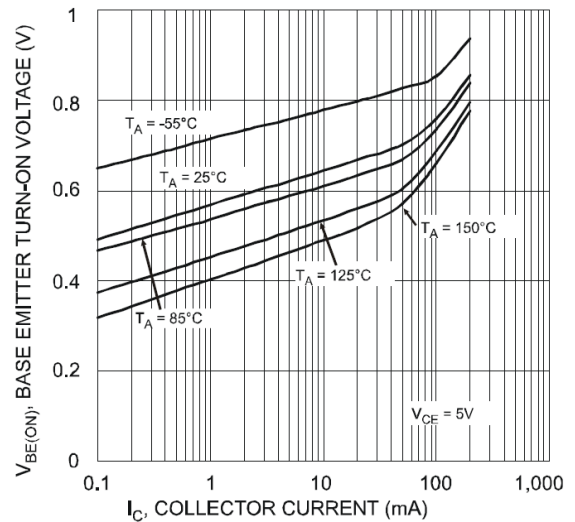
Typical Base Emitter Turn-On Voltage vs. Collector Current
