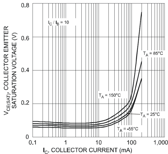
Typical Collector Emitter Saturation Voltage vs. Collector Current
