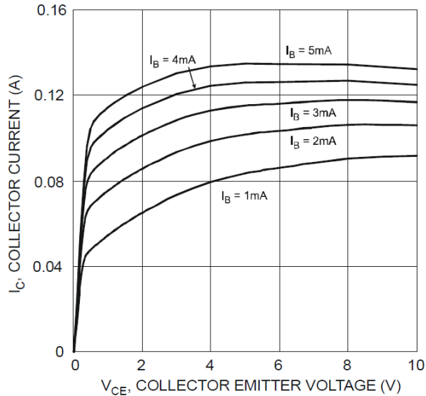
Typical Collector Current vs. Collector Emitter Voltage
