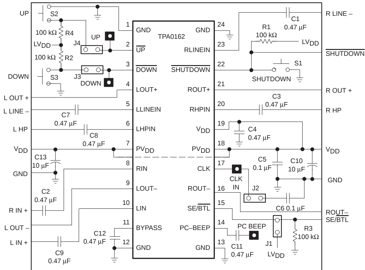
Figure 3–3. TPA0162 EVM Schematic Diagram
