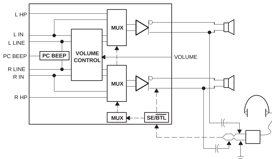
Figure 3–4. TPA0162 Amplifier IC
