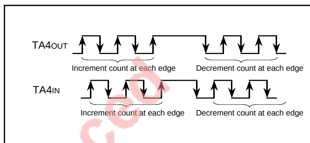
Fig. 20 Two-phase pulse signal processing operation of timer A4
