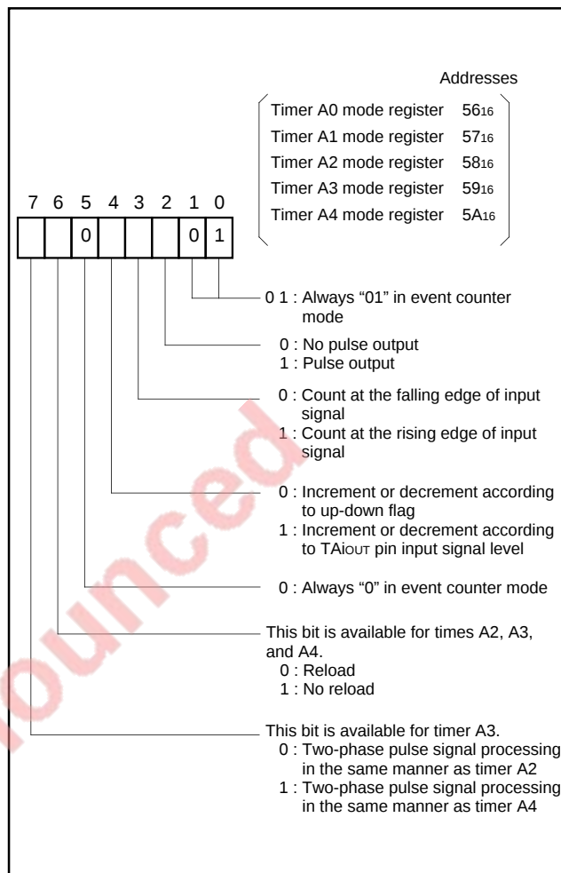
Fig. 17 Timer Ai mode register bit configuration during event counter mode
