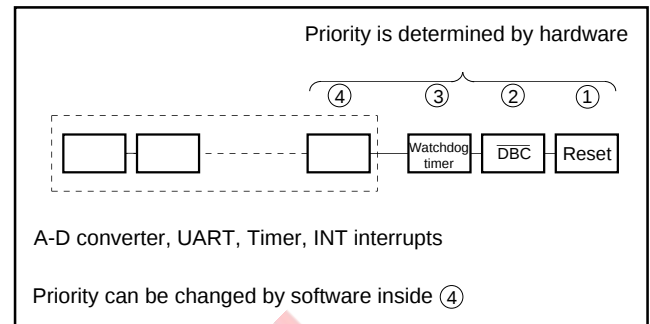
Fig. 7 Interrupt priority
