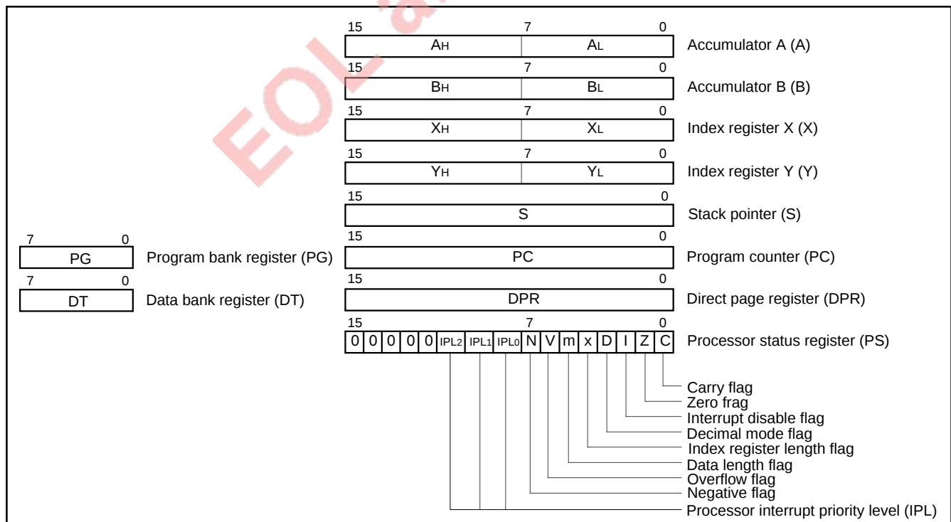
Fig. 3 Register structure
