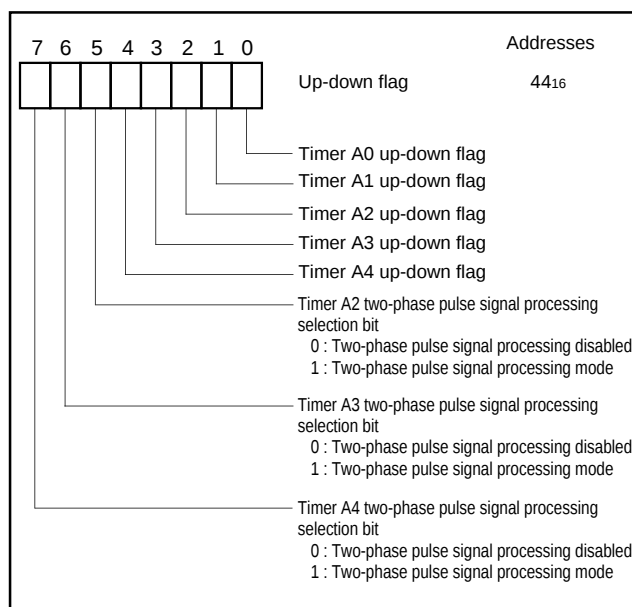
Fig. 18 Up-down flag bit configuration
