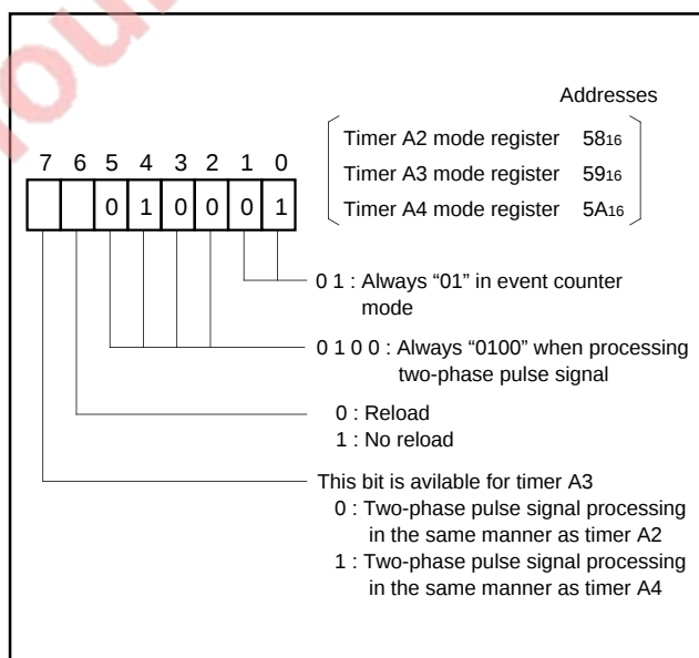
Fig. 21 Timer A j mode register bit configuration when performing two-phase pulse signal processing in event counter mode
