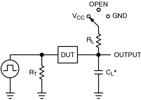
Figure 3. Test Circuit
