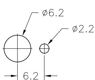
PANEL CUTOUT USING RING
