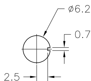
PANEL CUTOUT
