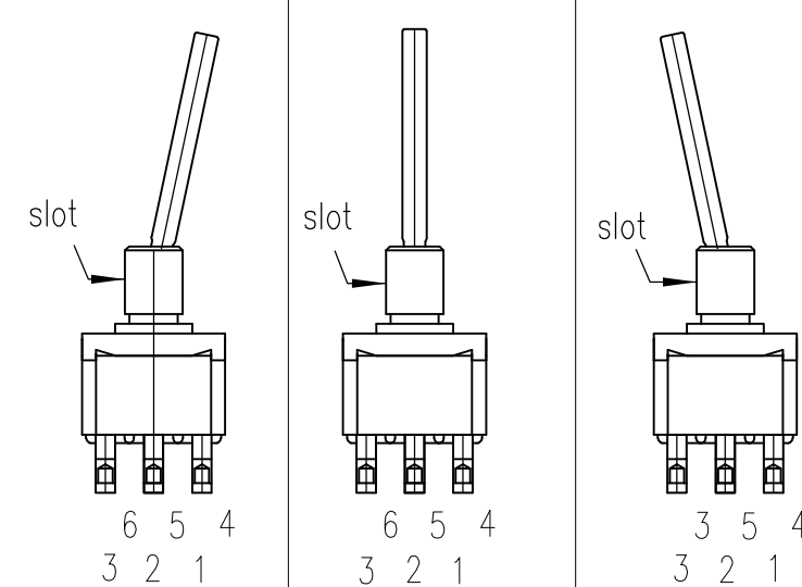
FUNCTION CHART
