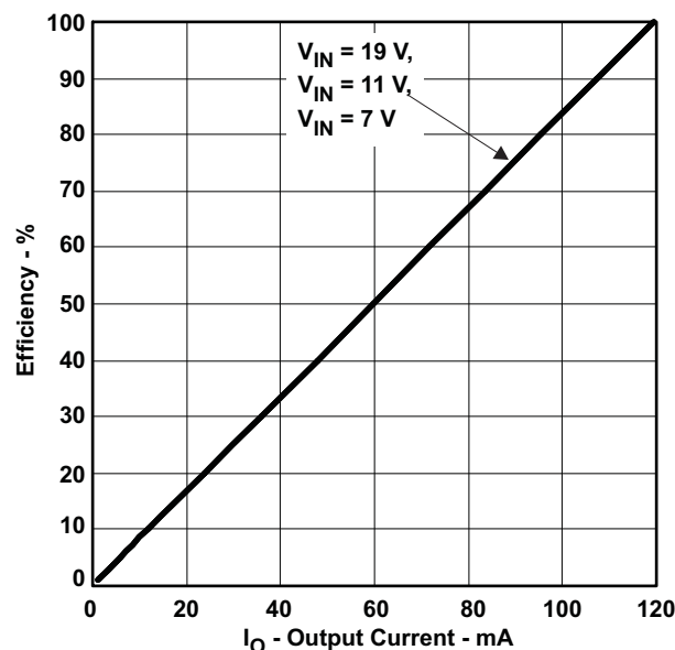
Figure 2. Dimming Linearity
