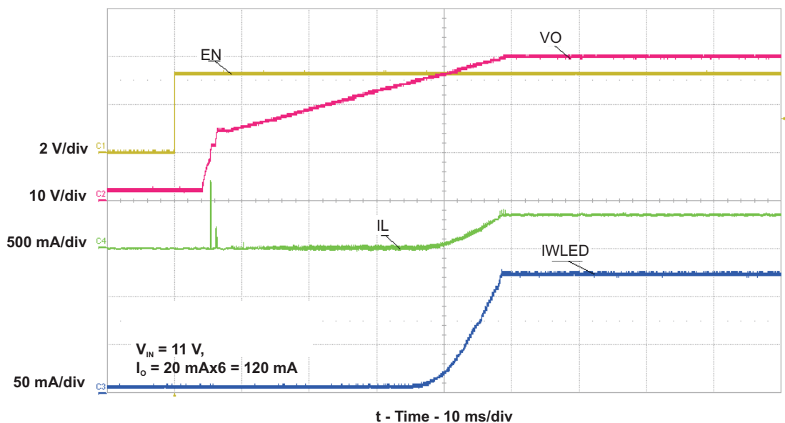
Figure 3. Start-up
