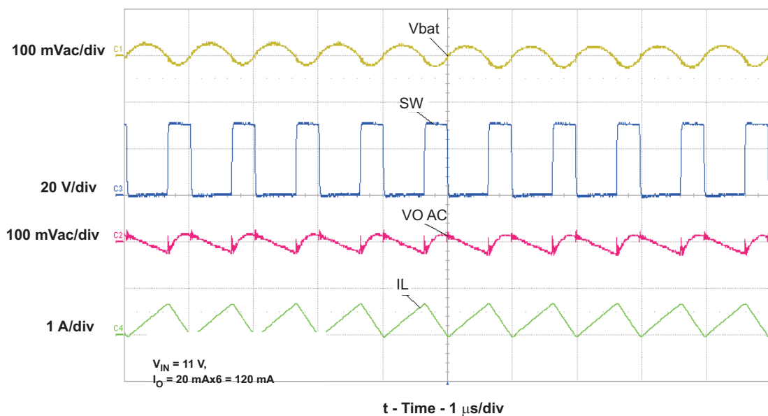
Figure 4. Switching Waveform
